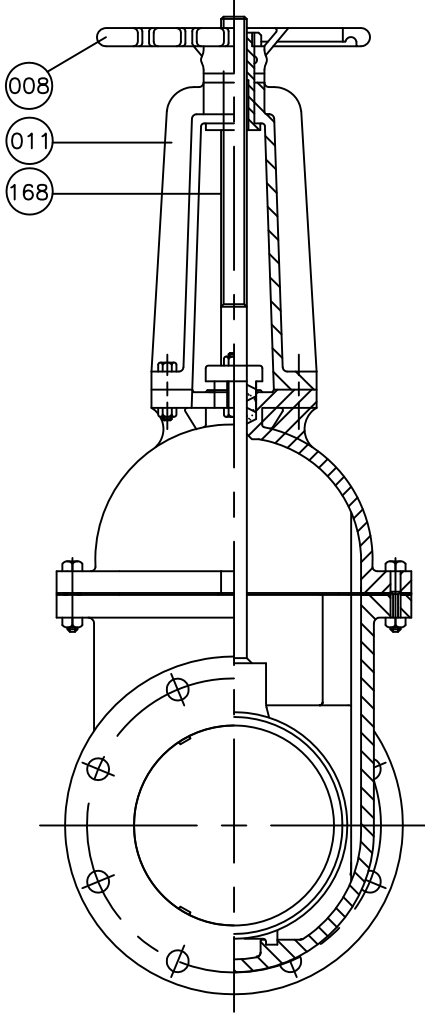
Yoke Construction For size 3"
