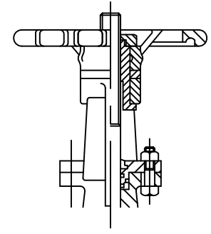
Yoke Construction For size 3"
